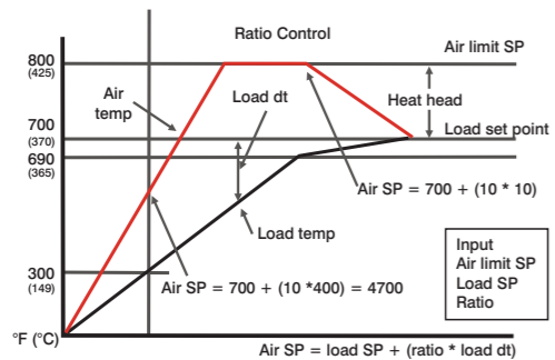
Air-to-work ratio control Consult SECO/WARWICK for the adjustable ratio system
