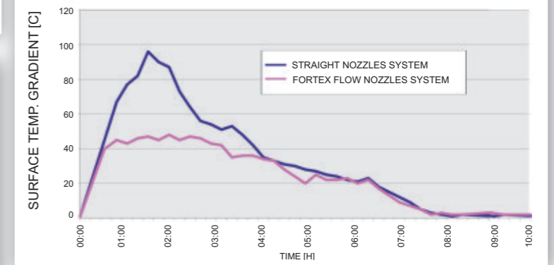
Temperature uniformity profiles
